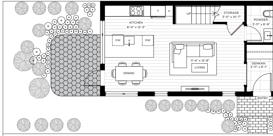
Level 1: 534 SF
