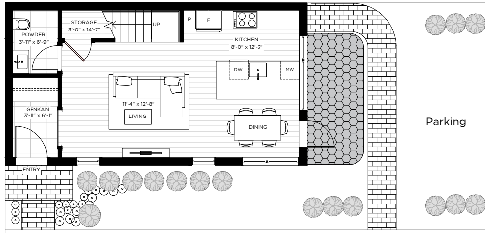
Level 1: 534 SF
