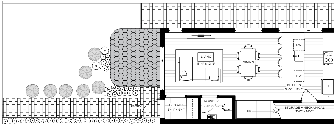
Level 1: 534 SF
