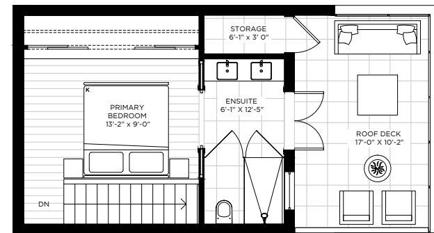
Level 3 (Interior): 348 SF
