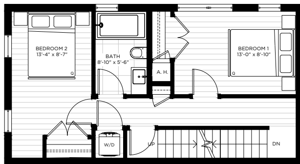
Level 2: 528 SF
