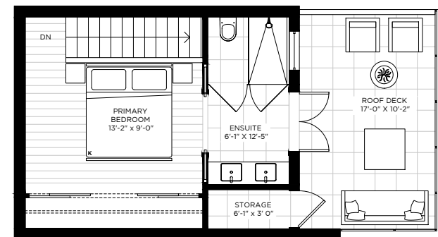
Level 3 (Interior): 348 SF
